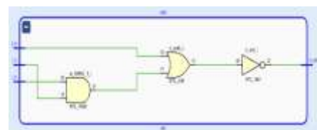
Figure.5 Schematic AOI
