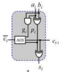
Figure.1 Generalized AOI
