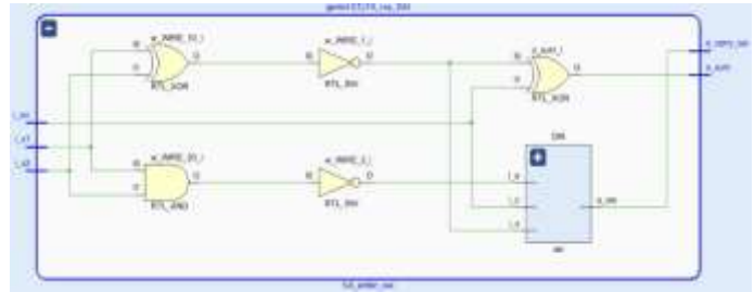
Figure.8 Schematic Full Adder OAI
