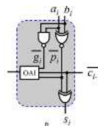
Figure.2 Generalized OAI
