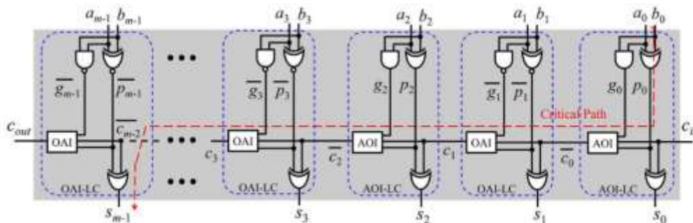
Figure.3 Proposed m-bit RCA design
