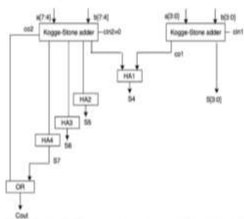
Figure 3. Block diagram of CIA_KOGGE-STONE(8-bit)
