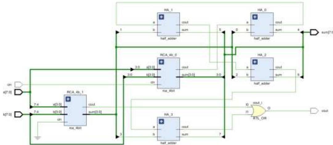
Figure.7 Schematic _CIA_RCA_8
