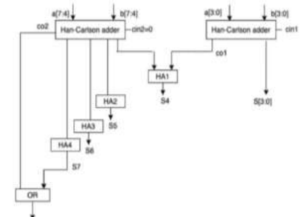
Figure 4. Block diagram of CIA_HAN-CARLSON(8-bit)
