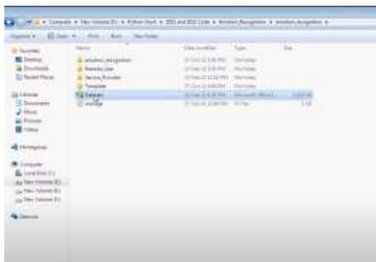
Fig.4. Dataset details.
