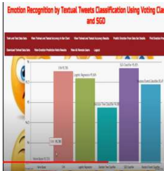
Fig.6. Output results.
