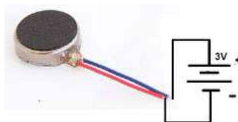
Fig5: Vibration motor
