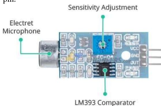
Fig 3: Sound Sensor
