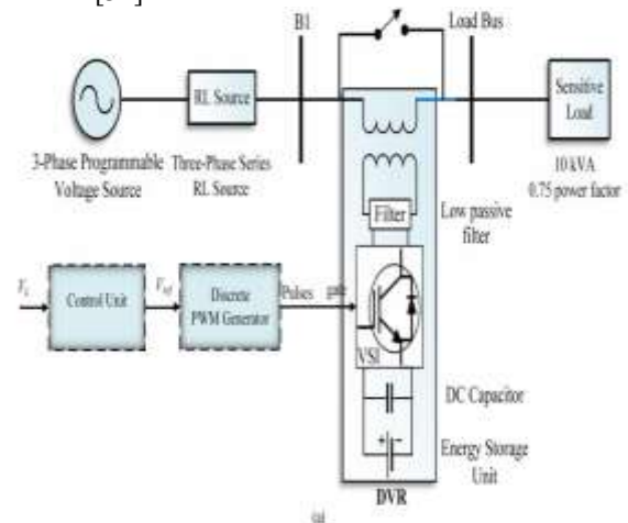
FIGURE 8. (a) Single line diagram of test system with DVR
