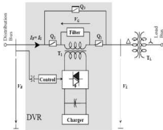
FIGURE 3. Principle design of DVR connected at distribution end [15].
