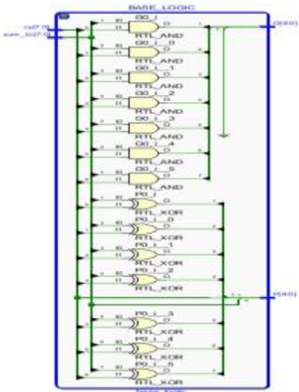
Figure.5 Base Logic
