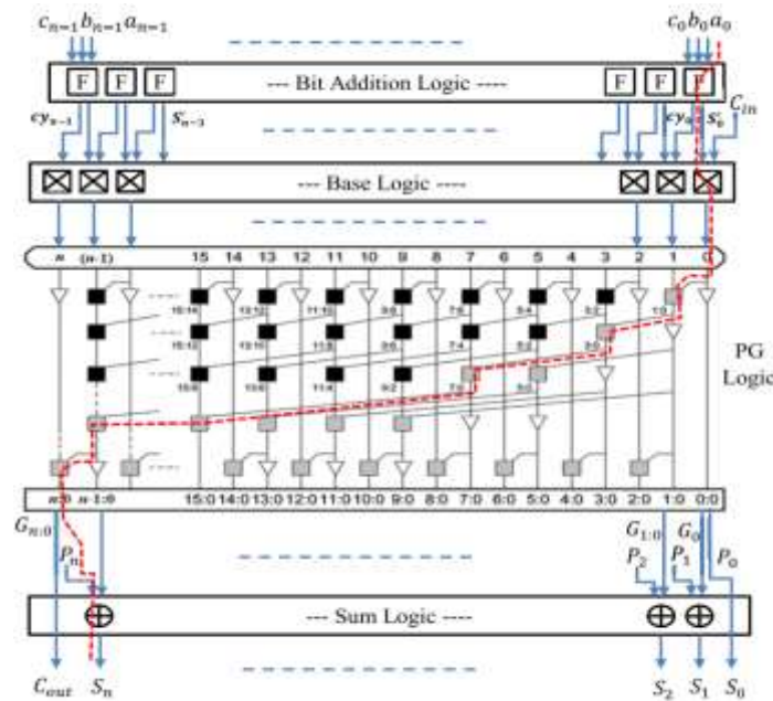
Figure.1 Proposed three adder operand
