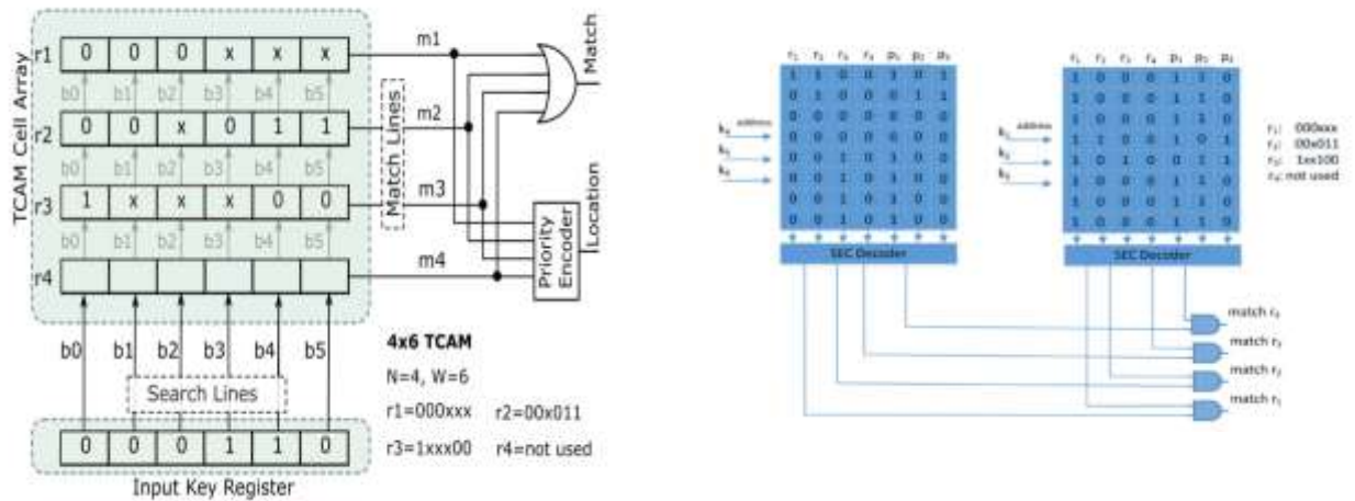
Figure.1 Emulating TCAMs with memory Figure.2 Error detection & correction using SEC decoder
