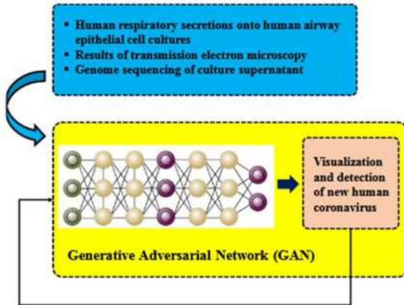
Fig 2: GAN network
