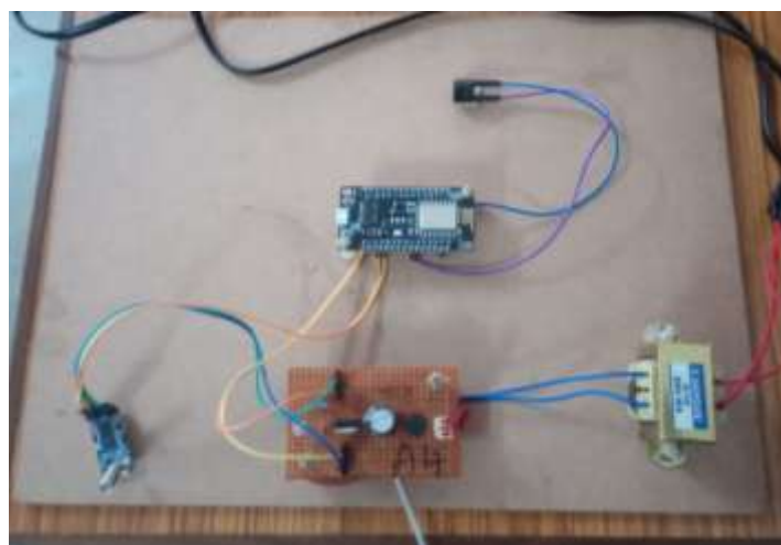
Figure.6 Working kit
