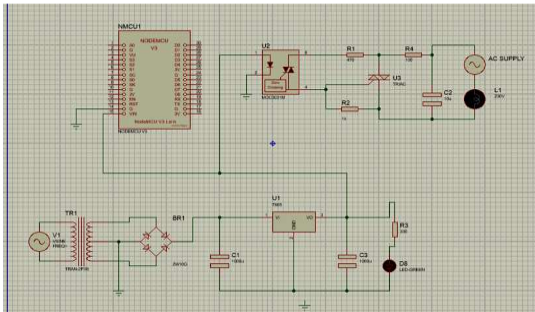
Figure.2 Schematic Diagram
