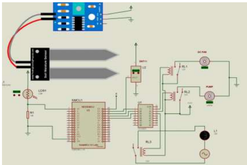
Figure.2 Schematic Diagram
