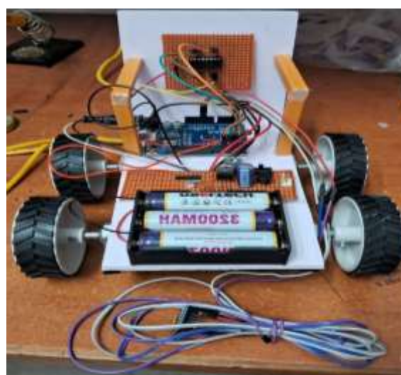
Figure.3 Working kit
