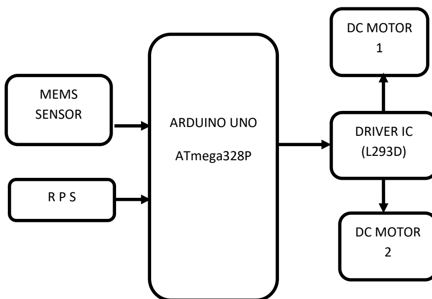
Figure.1 Block diagram
