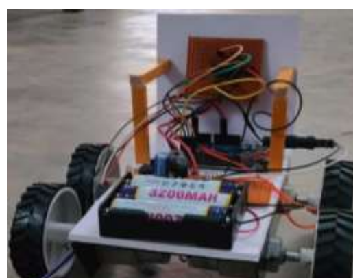
Figure.3 Working kit
