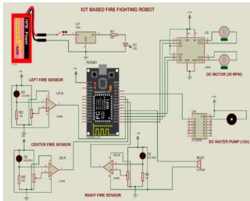
Figure.2 Schematic Diagram
