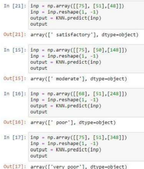
Fig.2. Output results.
