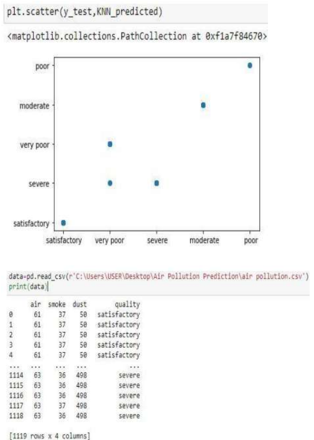
Fig.1. Dataset details.
