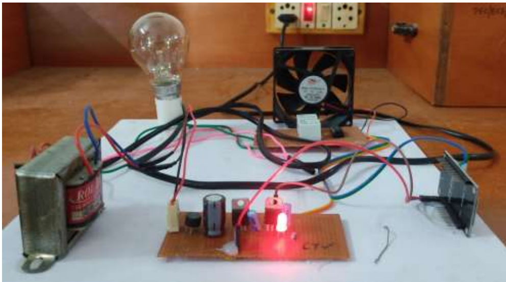
Figure.3 Working Kit
